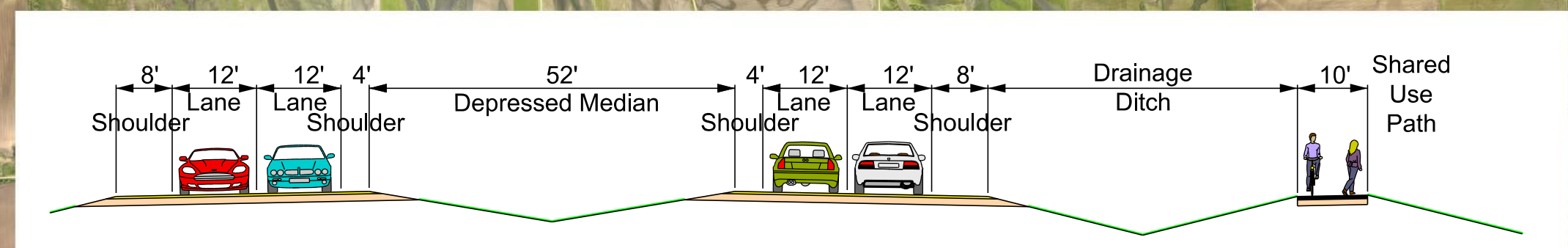
Option A: US 14 Alignment
